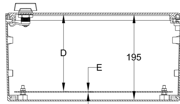
SEC. A-A'
